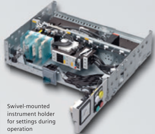
Miniature withdrawable unit, size \frac{1}{2} , height 200 mm
