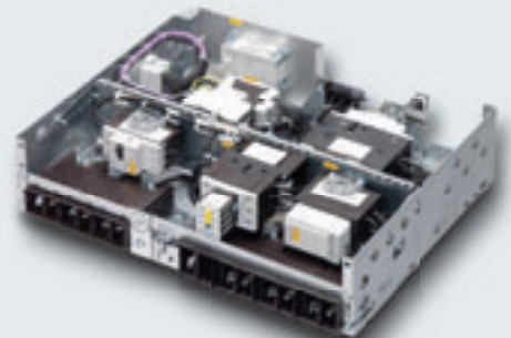
Standard withdrawable unit, height 150 mm (rear view)
