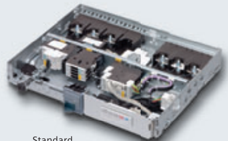
Standard withdrawable unit, height 100 mm
